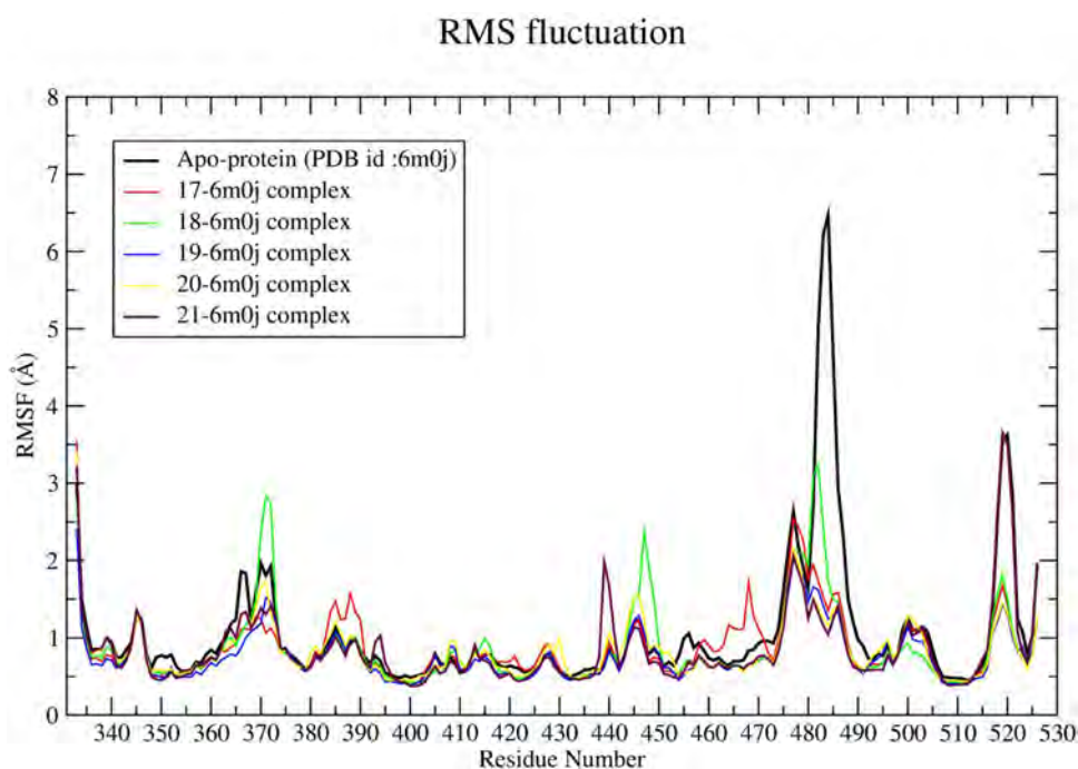
Figure 8. RMSF profile of apo-protein and ligand (17–21)-spike protein complexes.
